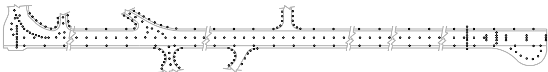
LIGHTING AIDS RWY 12/30 AND EXIT TWY
