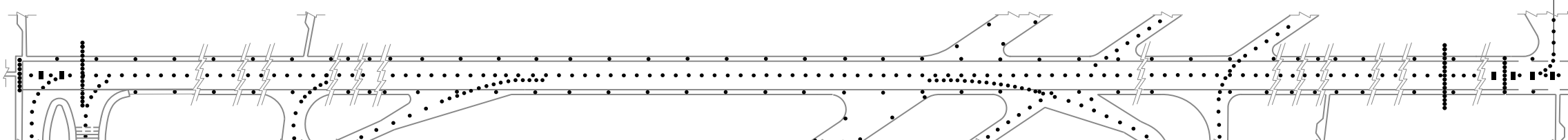
LIGHTING AIDS RWY 03/21 AND EXIT TWY
