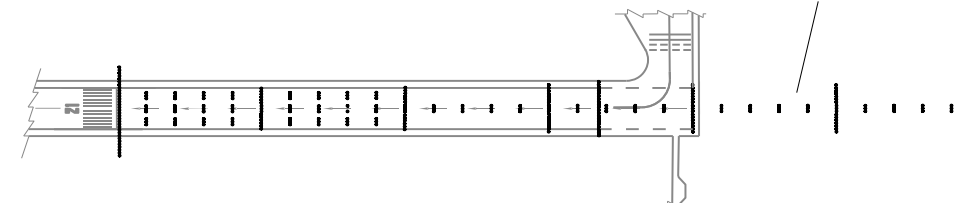
Precision approach CAT II/III lighting system
