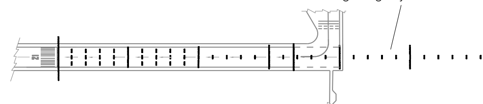
Precision approach CAT II/III lighting system
